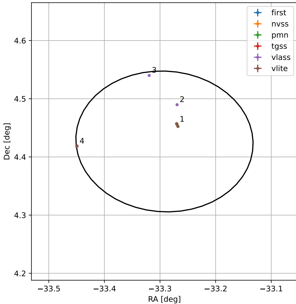
4FGL J2146.8+0425
