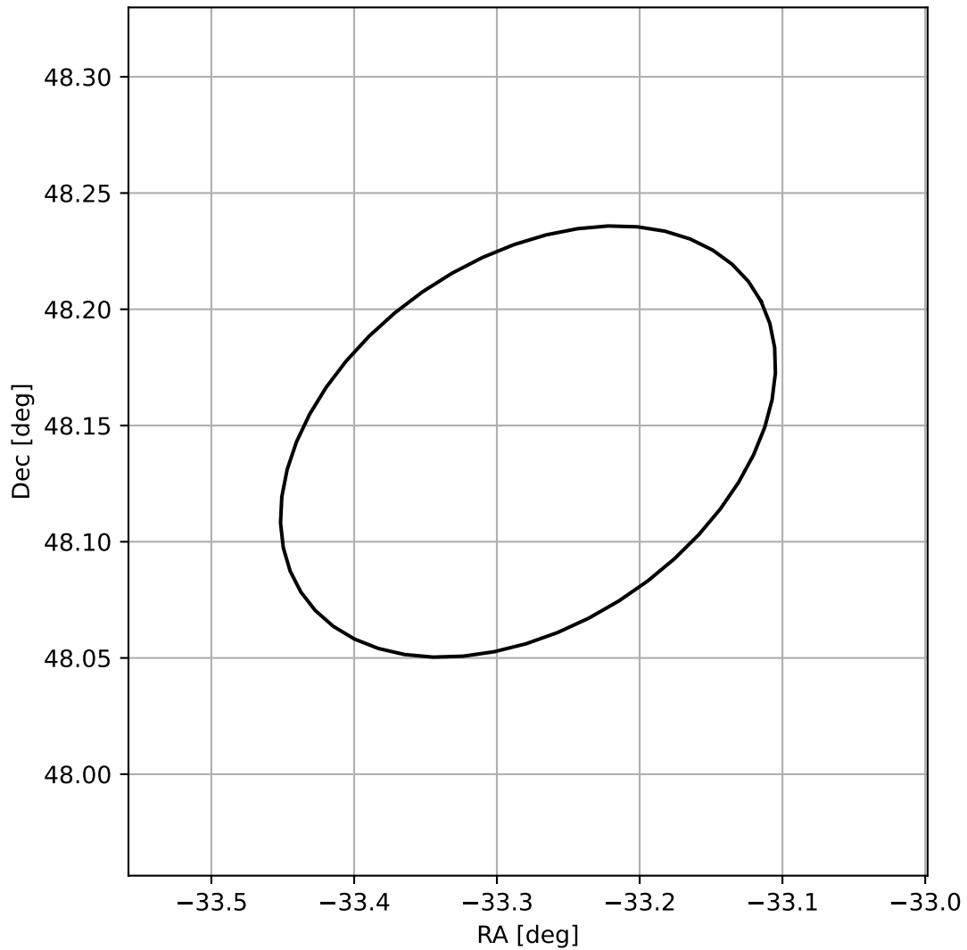
4FGL J2146.8+4808
