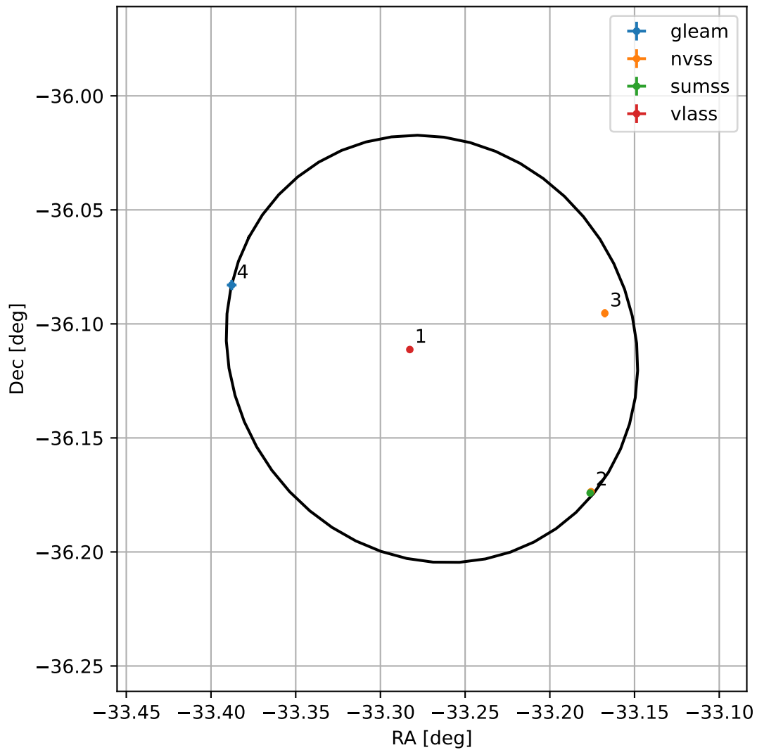
4FGL J2146.9-3606
