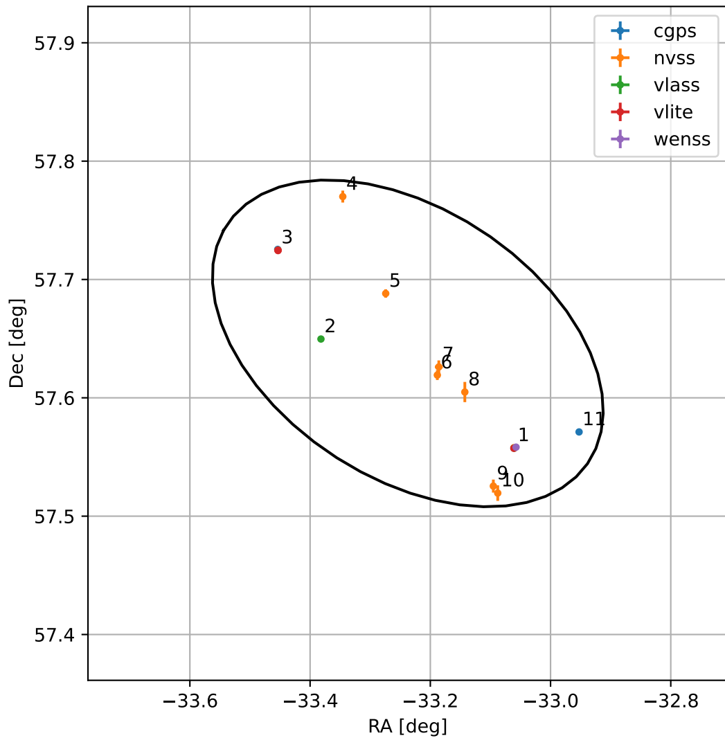
4FGL J2147.0+5738
