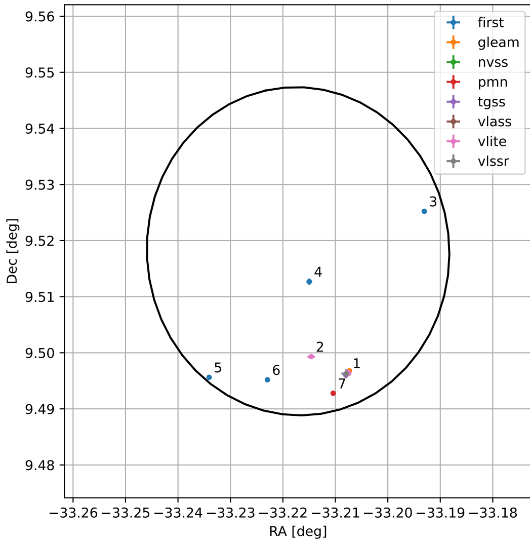
4FGL J2147.1+0931
