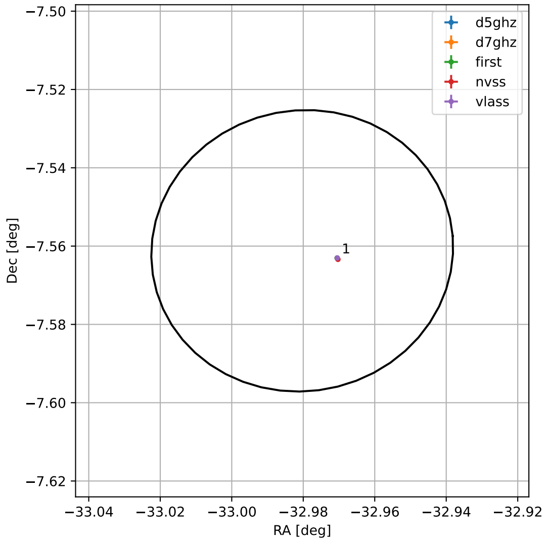
4FGL J2148.0-0733
