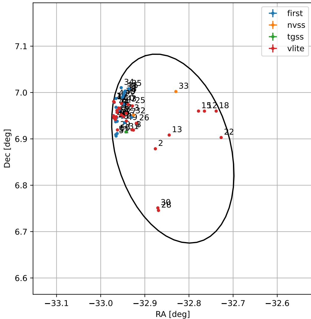
4FGL J2148.6+0652
