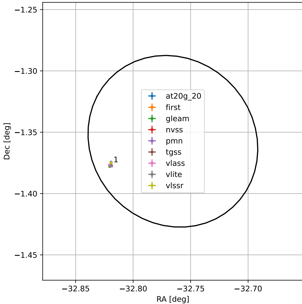
4FGL J2148.9-0121
