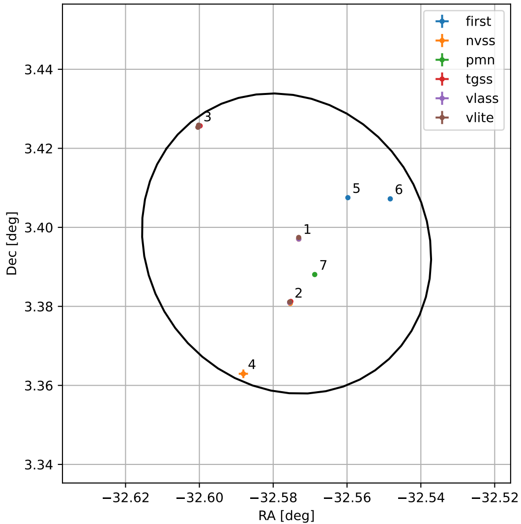
4FGL J2149.6+0323
