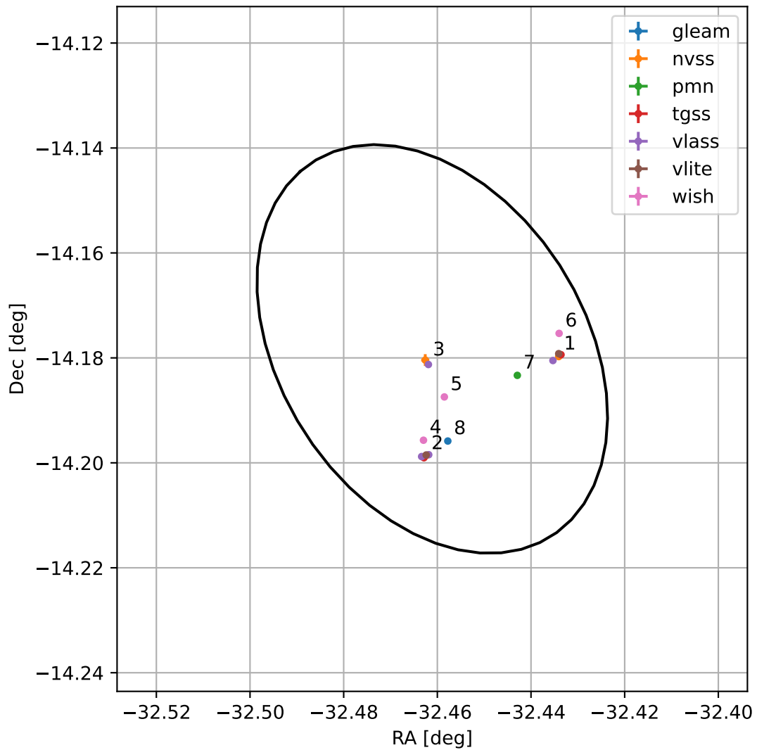
4FGL J2150.1-1410
