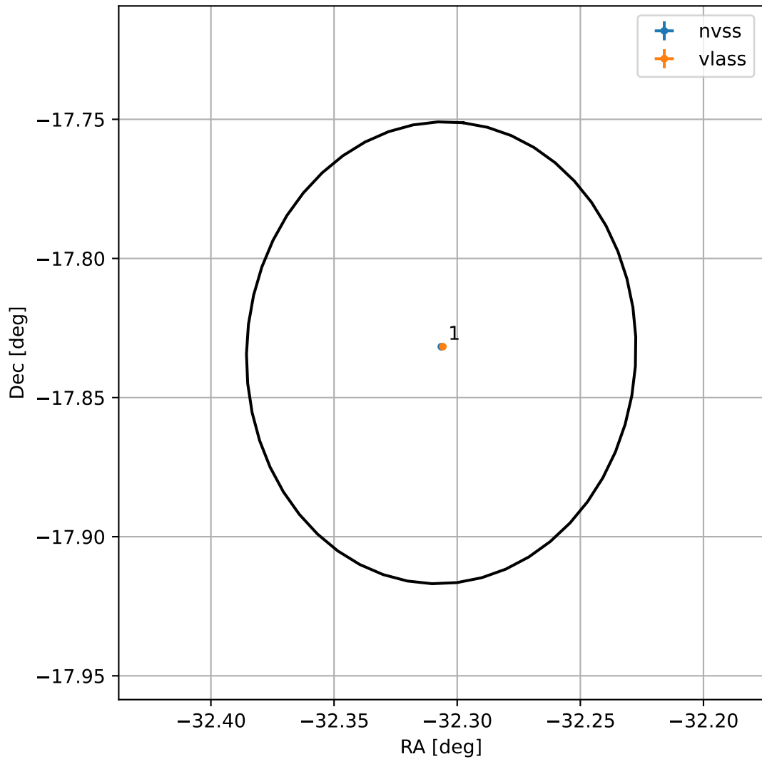
4FGL J2150.7-1750
