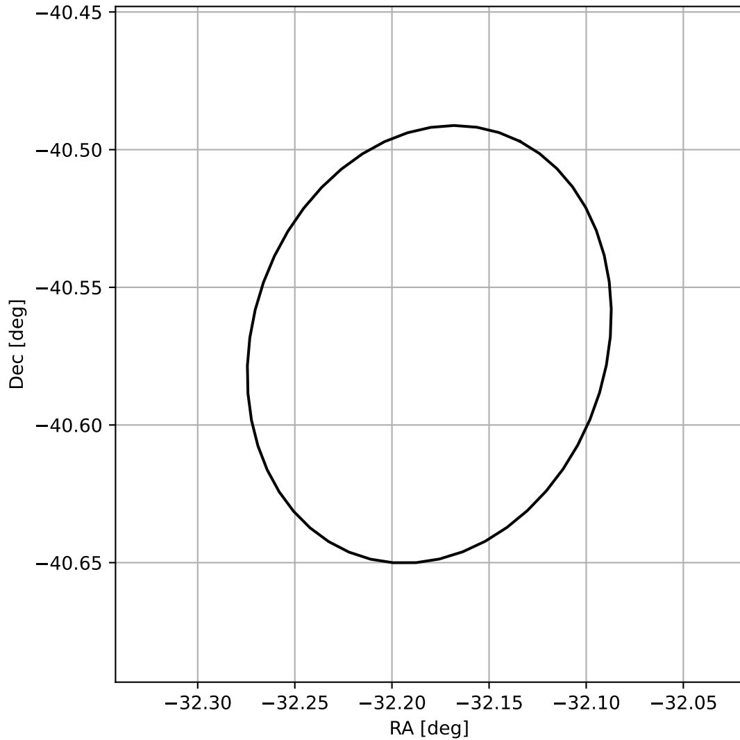
4FGL J2151.2-4034
