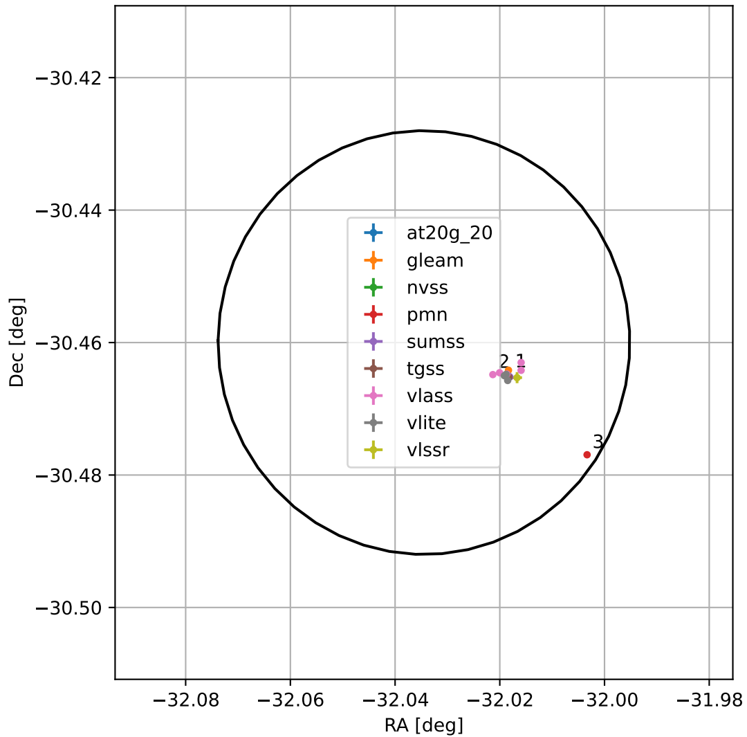
4FGL J2151.8-3027
