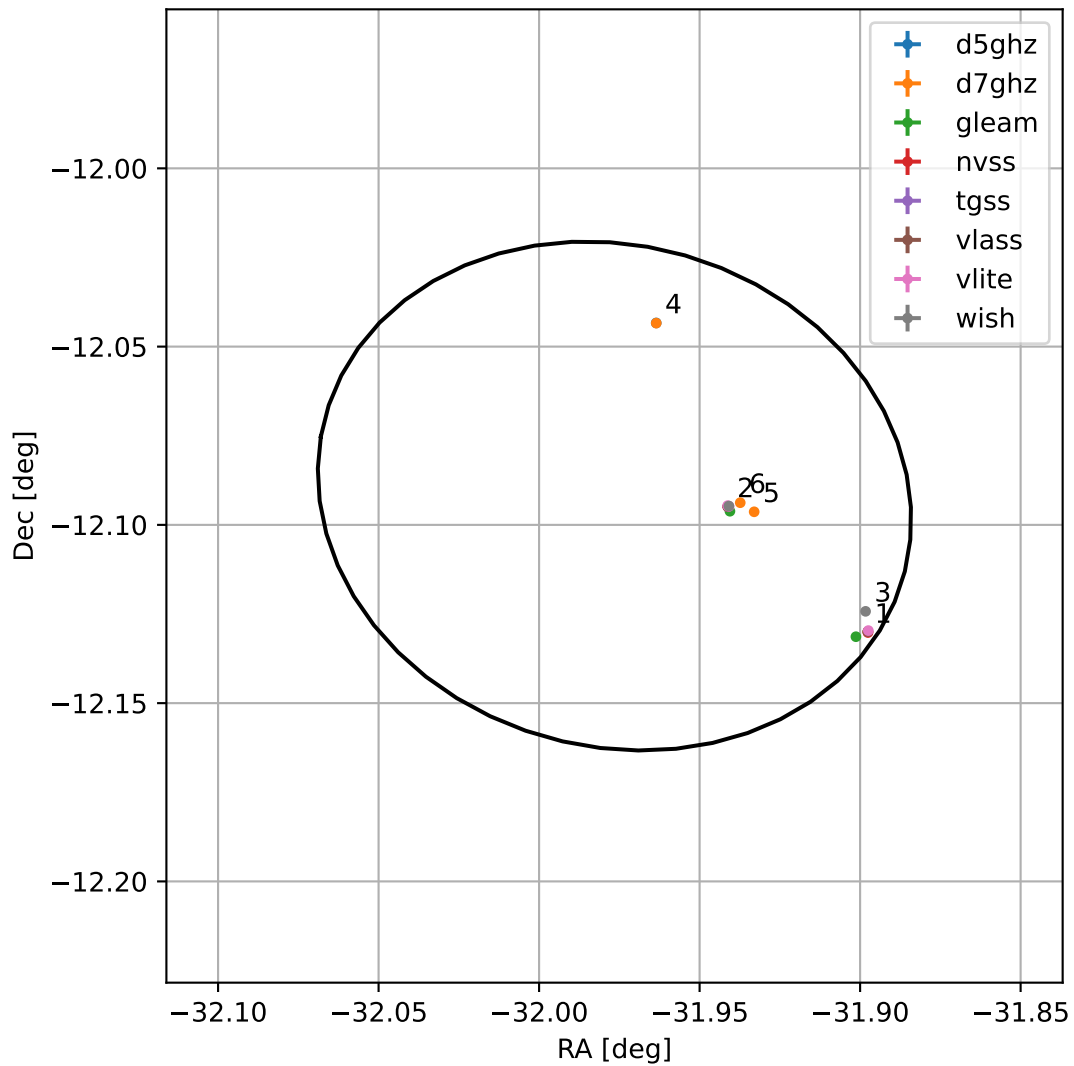
4FGL J2152.0-1205
