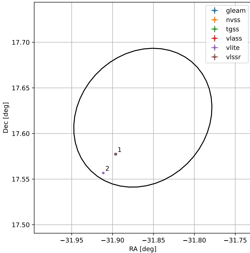
4FGL J2152.5+1737
