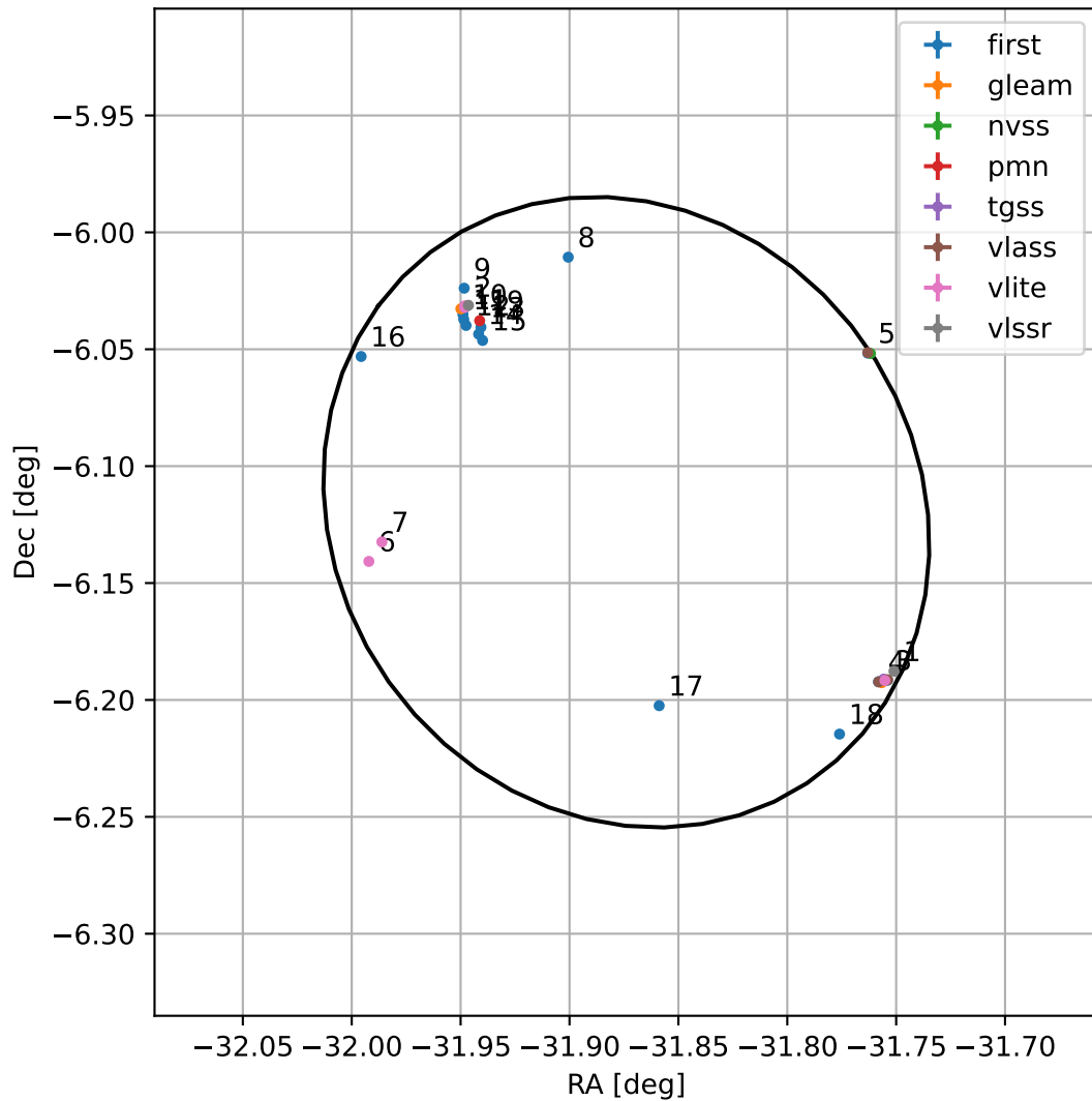
4FGL J2152.5-0607
