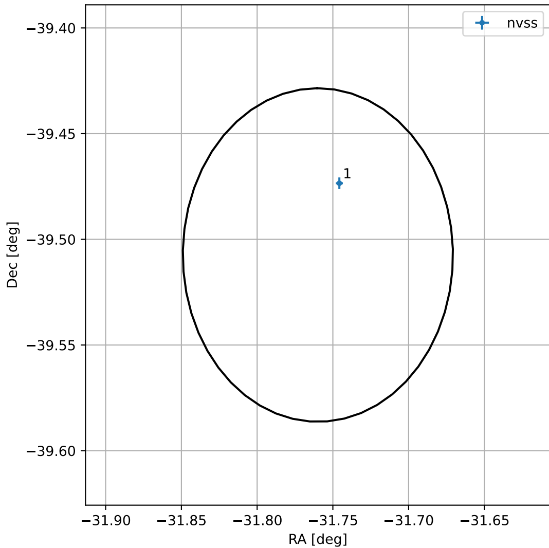
4FGL J2152.9-3930
