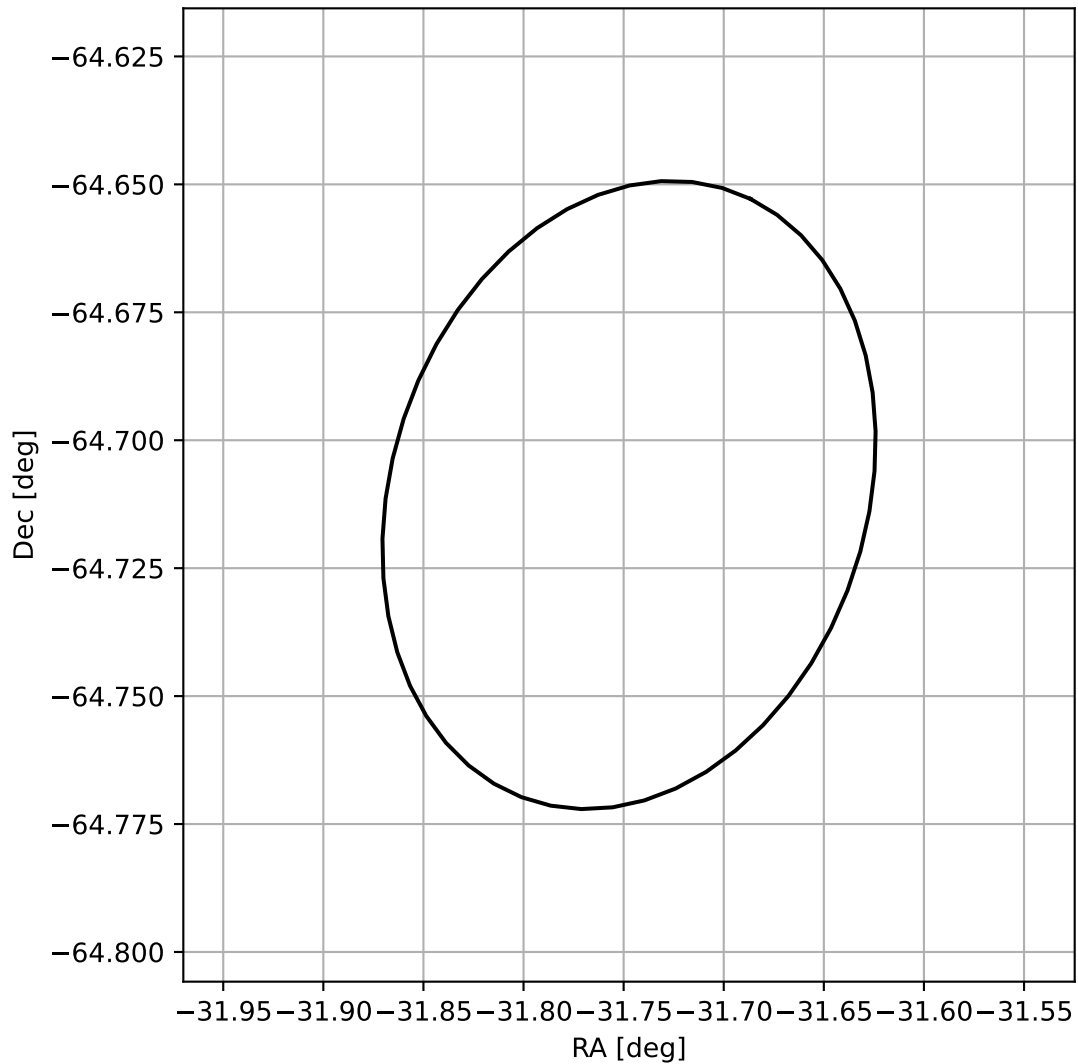
4FGL J2153.0-6442
