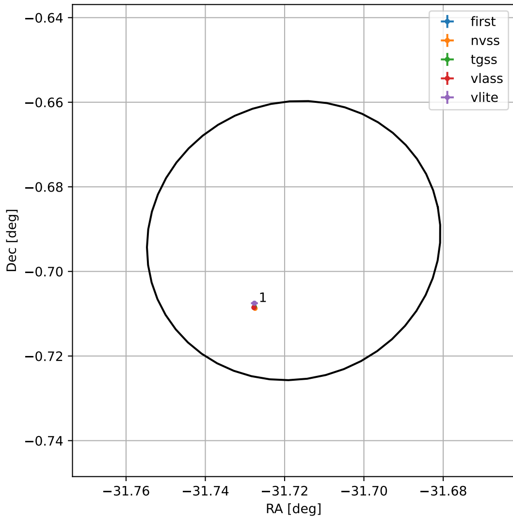
4FGL J2153.1-0041
