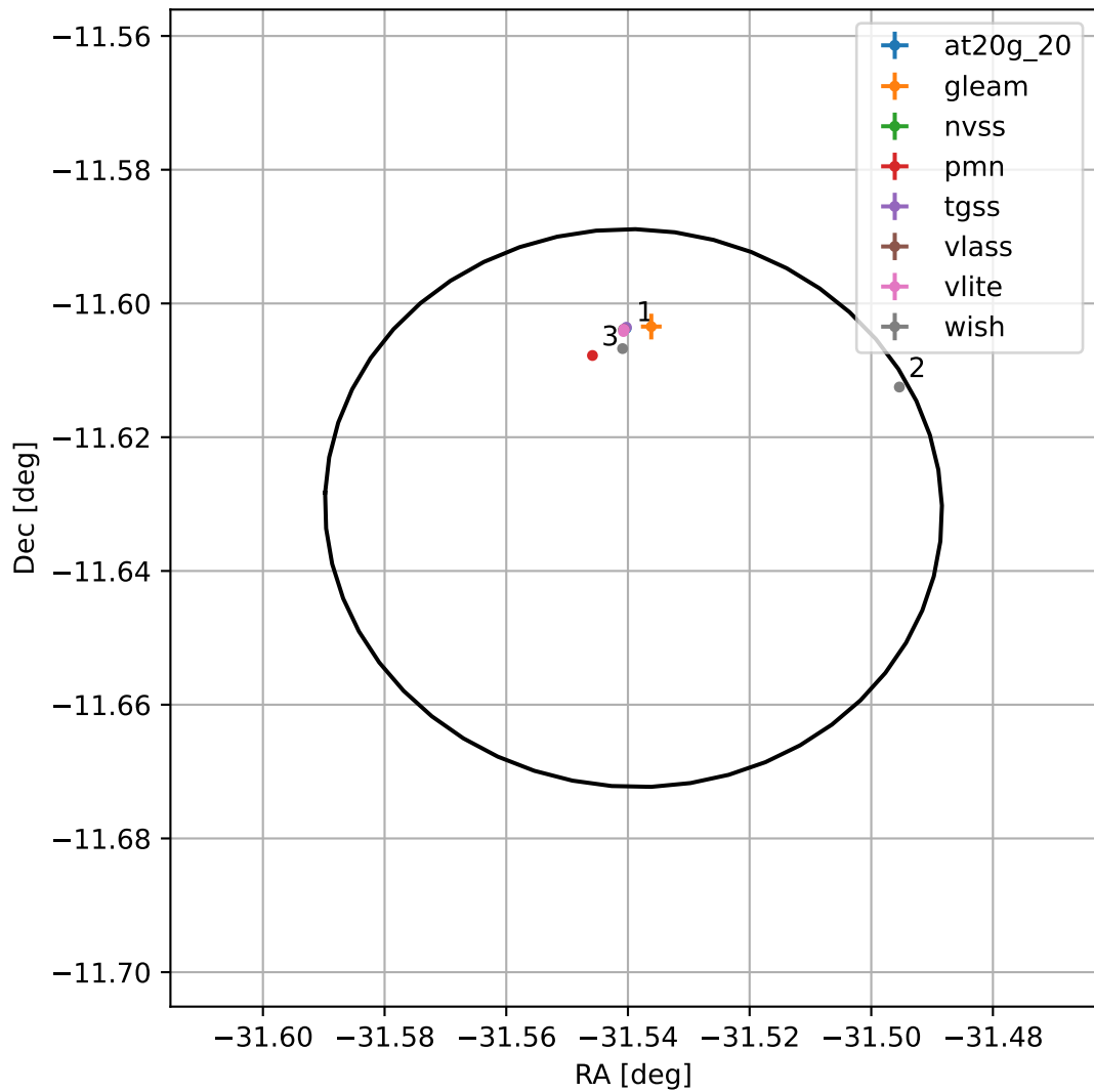
4FGL J2153.8-1137
