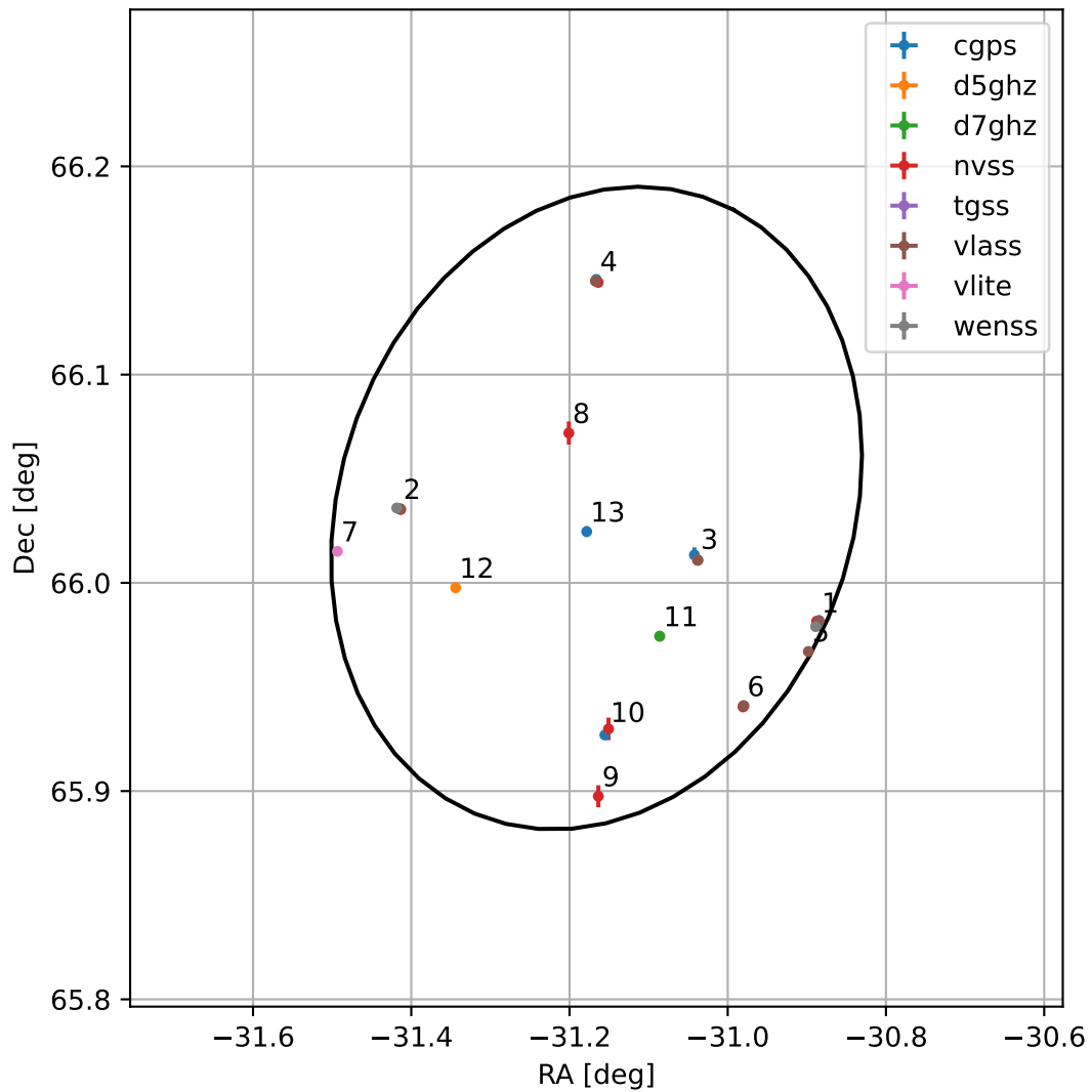
4FGL J2155.3+6602
