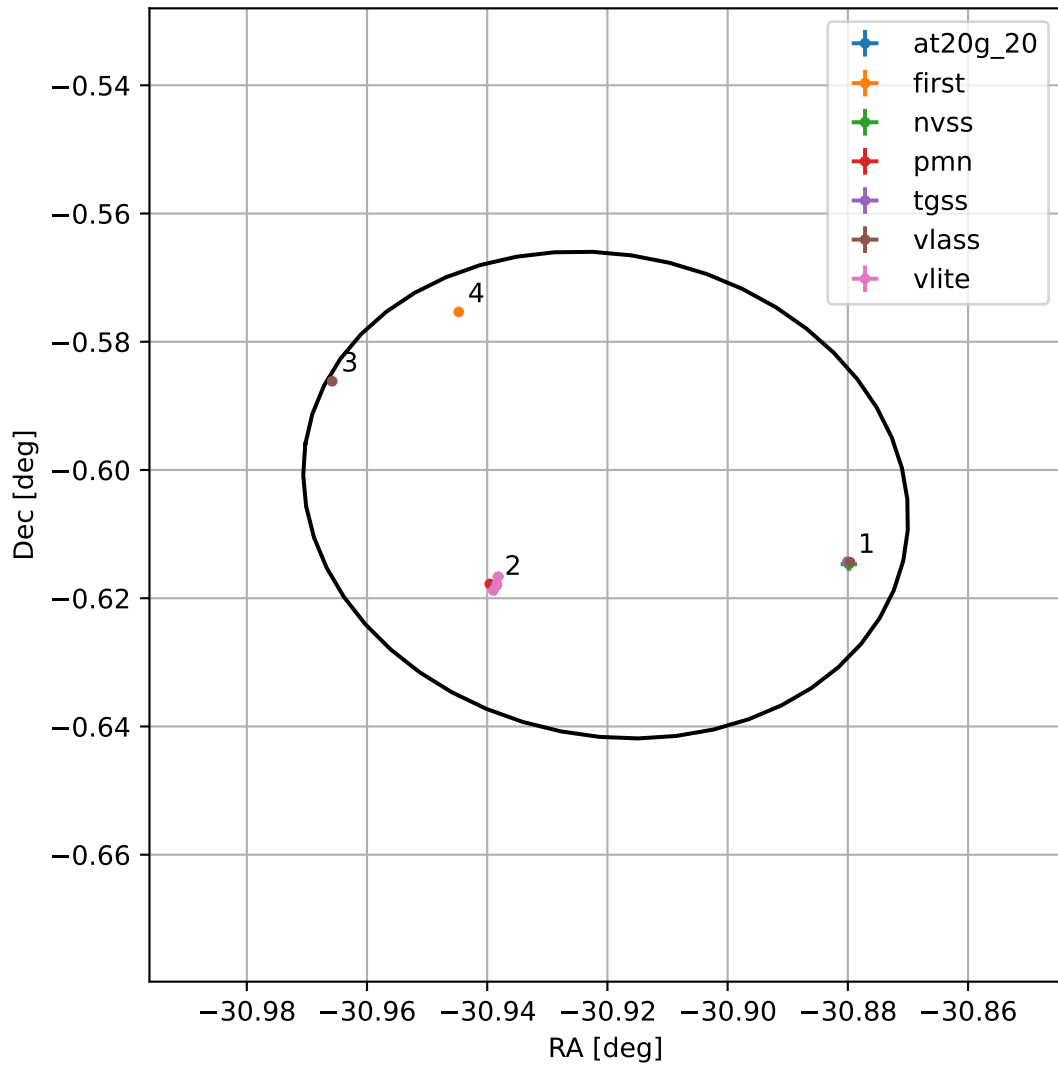
4FGL J2156.3-0036
