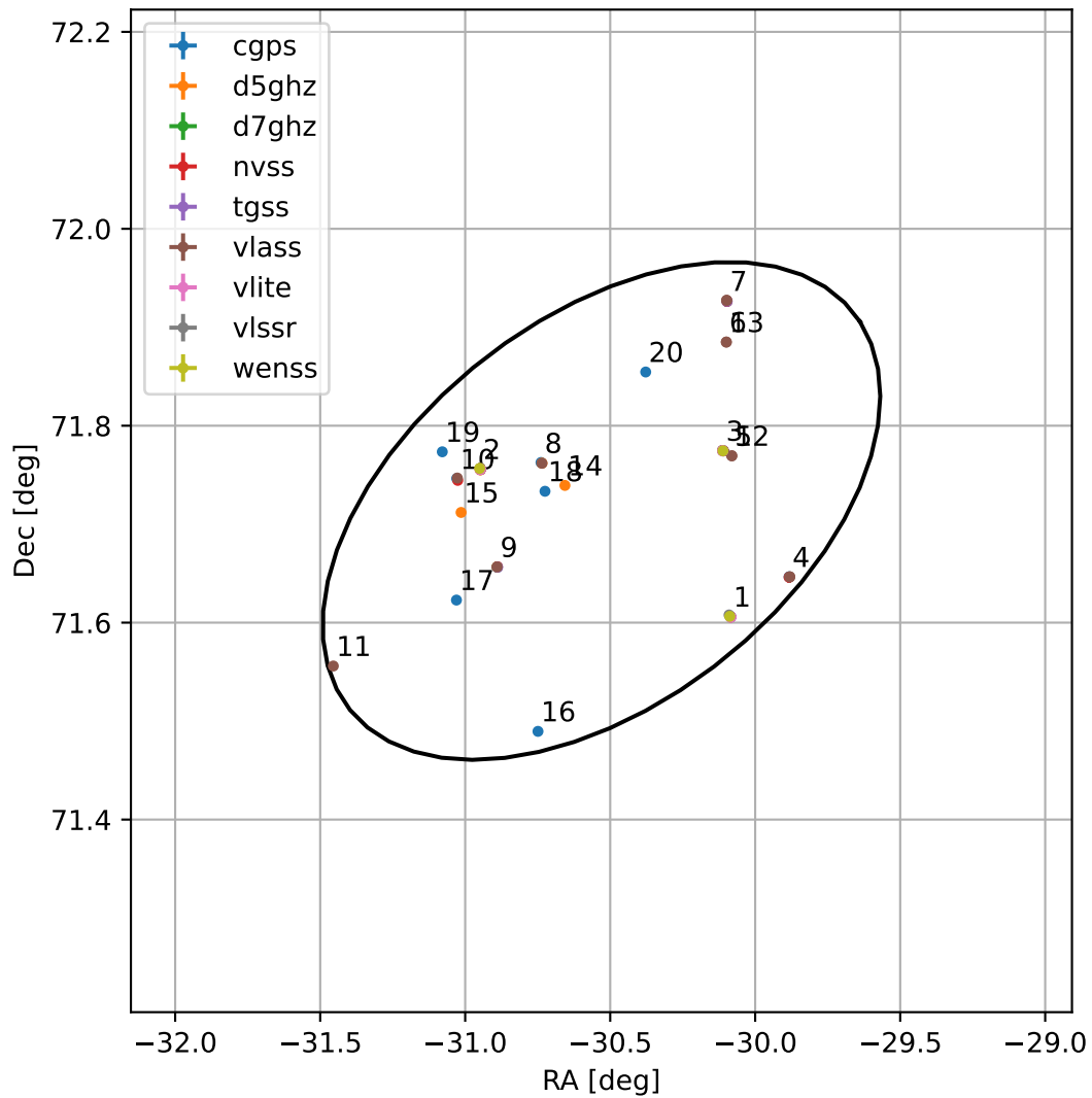
4FGL J2157.8+7142
