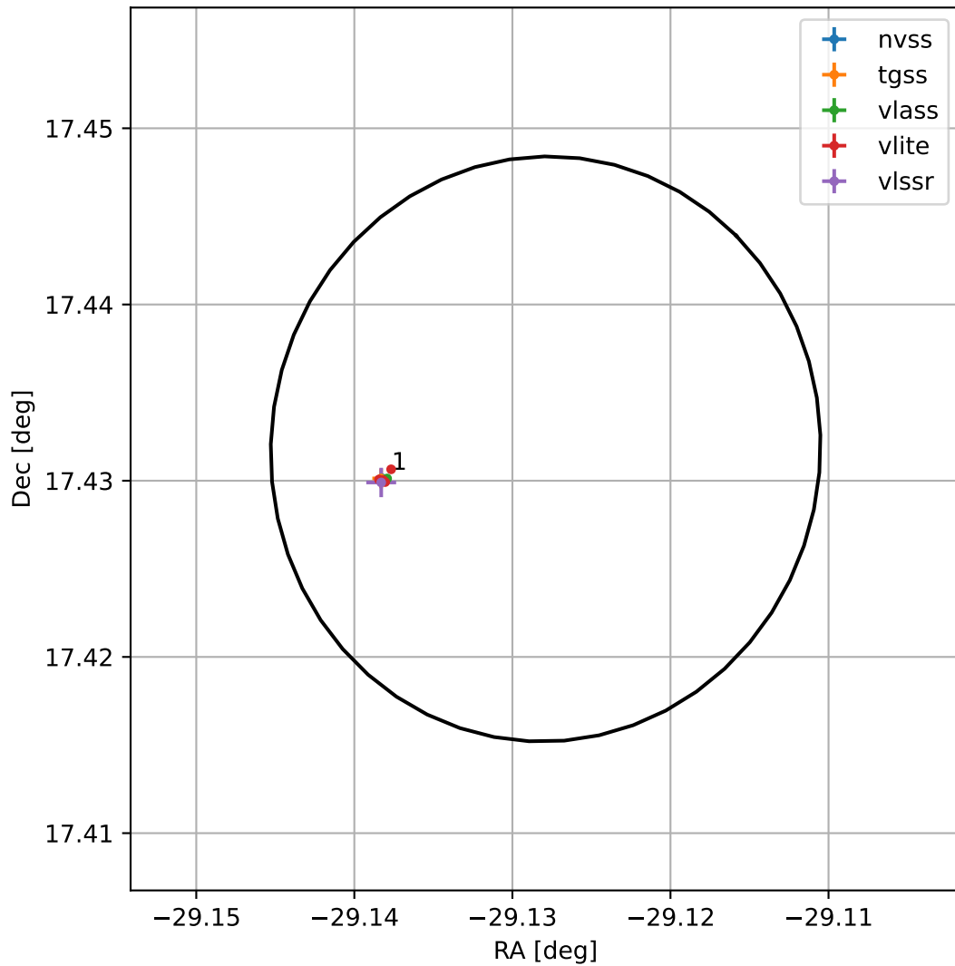
4FGL J2203.4+1725
