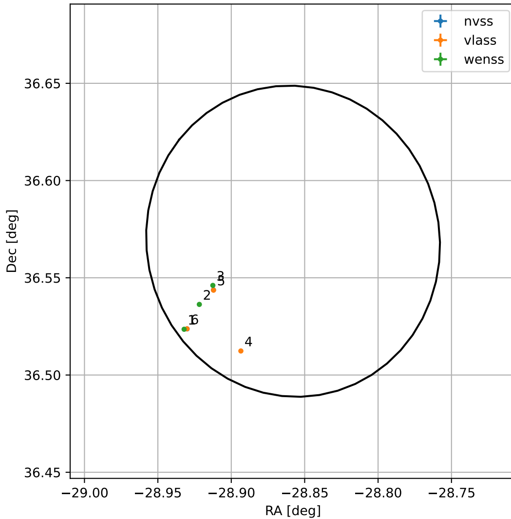
4FGL J2204.5+3634
