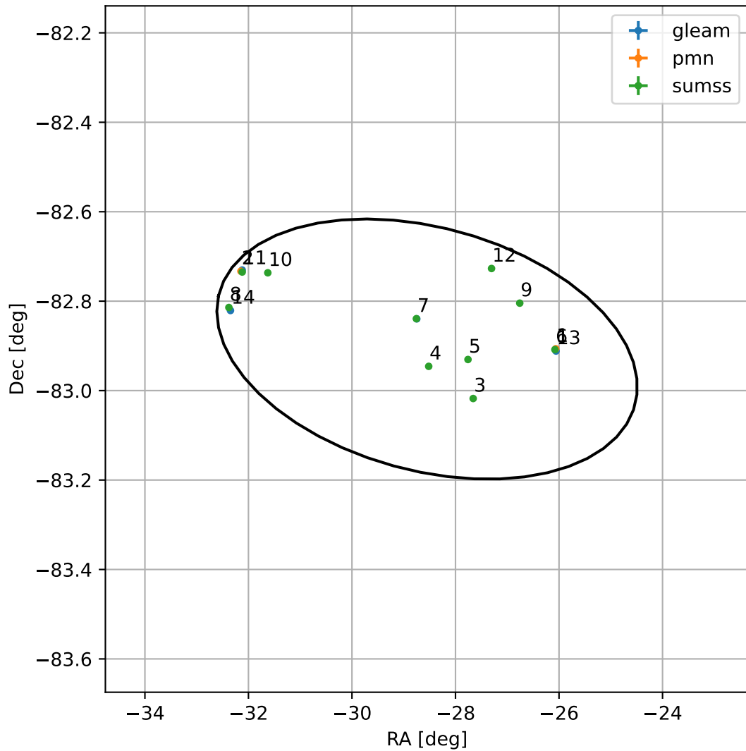
4FGL J2205.8-8254
