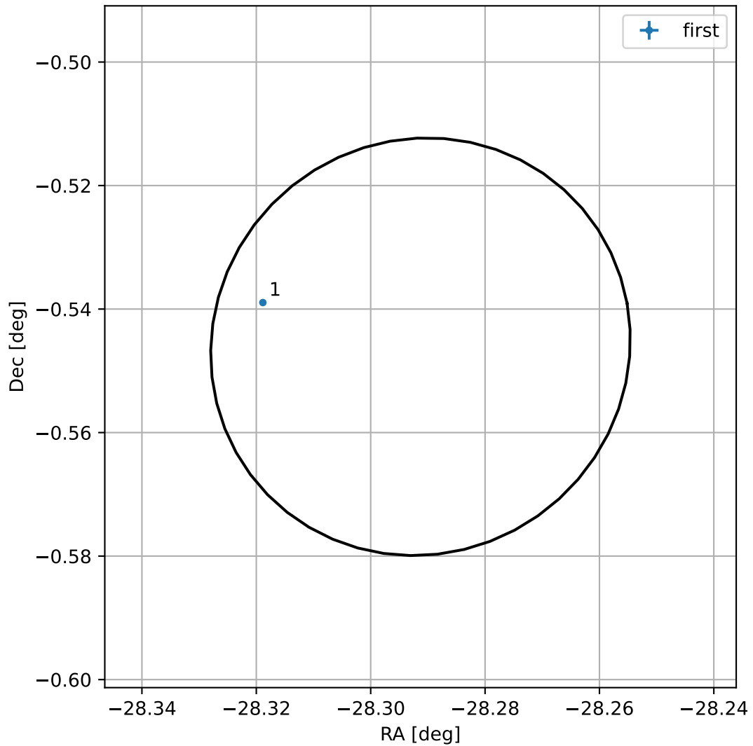
4FGL J2206.8-0032
