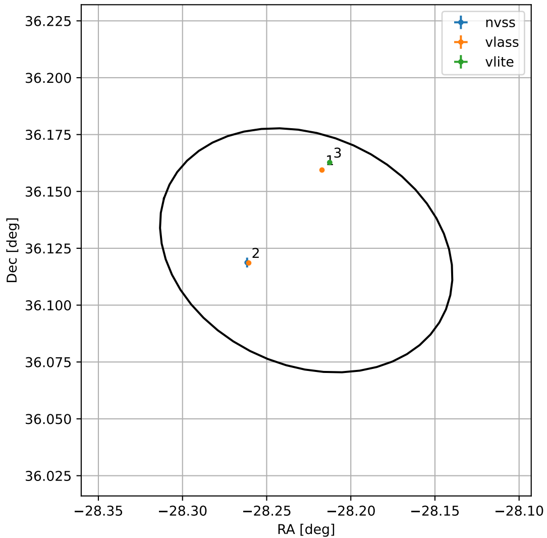
4FGL J2207.0+3607
