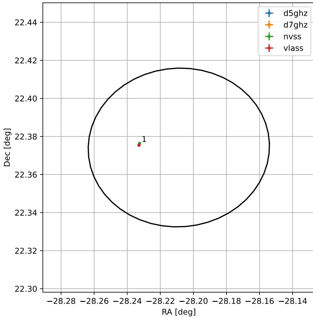
4FGL J2207.1+2222
