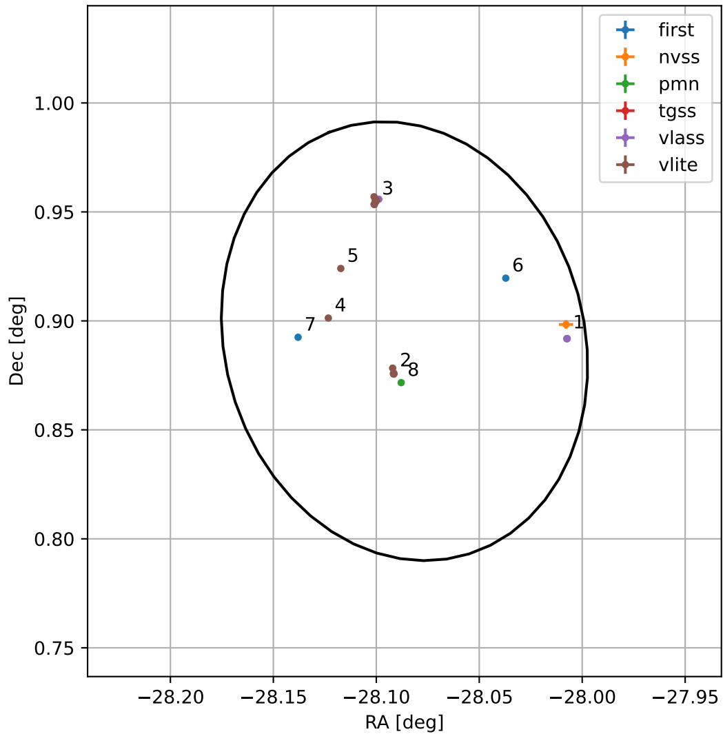
4FGL J2207.6+0053
