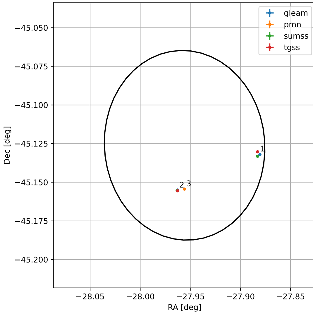
4FGL J2208.1-4507
