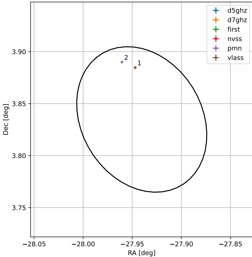
4FGL J2208.2+0350
