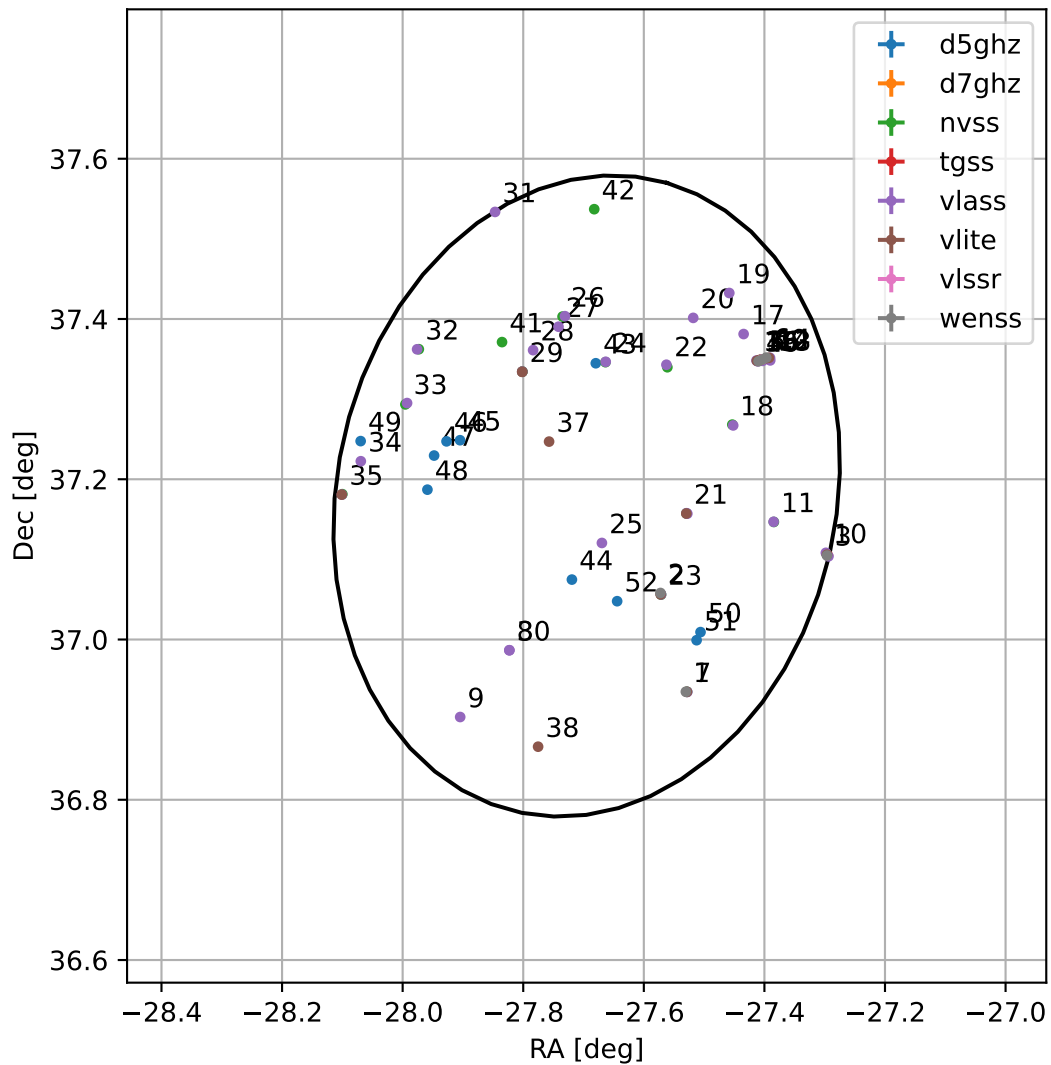
4FGL J2209.2+3710
