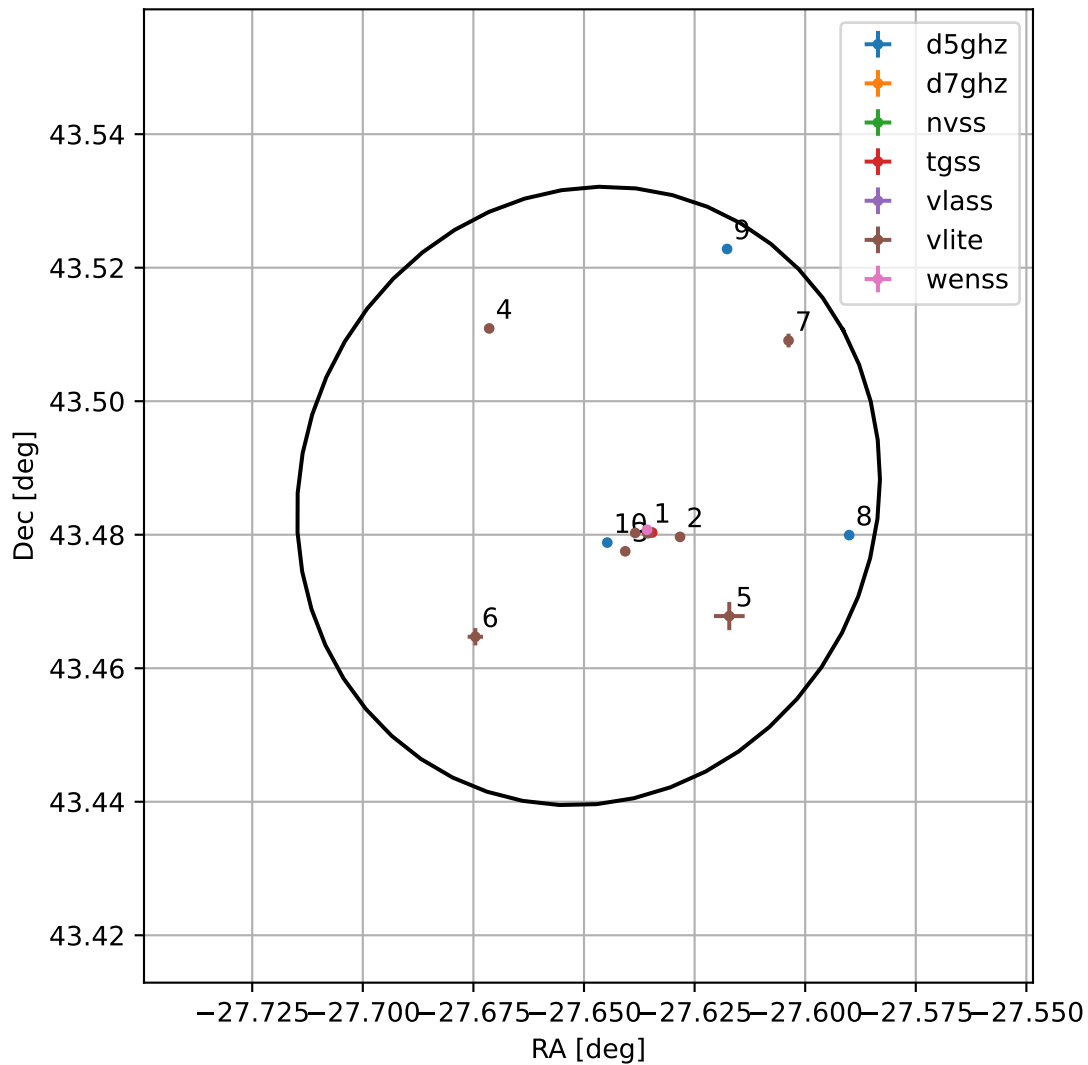
4FGL J2209.4+4329
