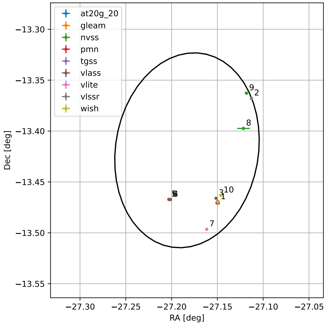
4FGL J2211.2-1325
