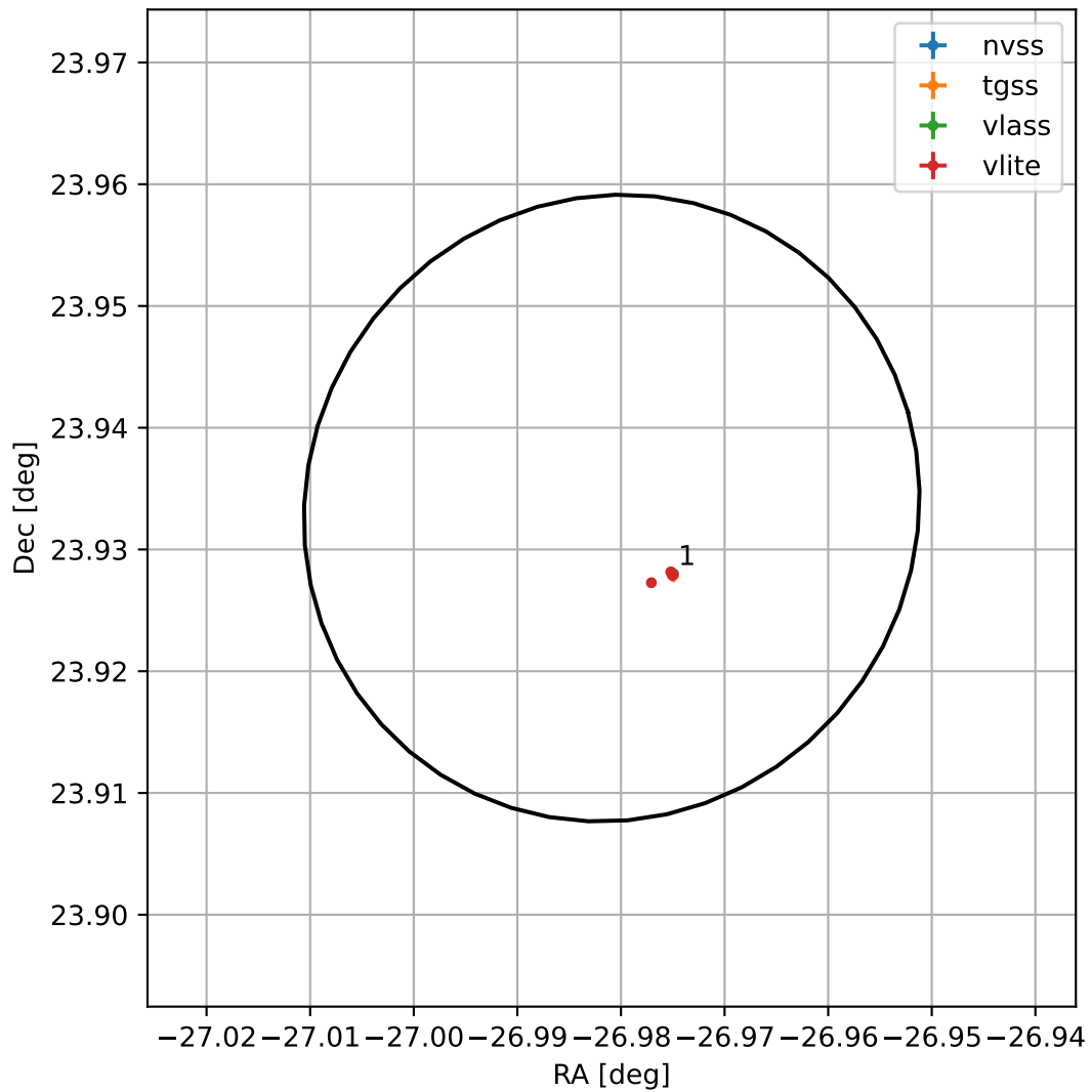
4FGL J2212.0+2356
