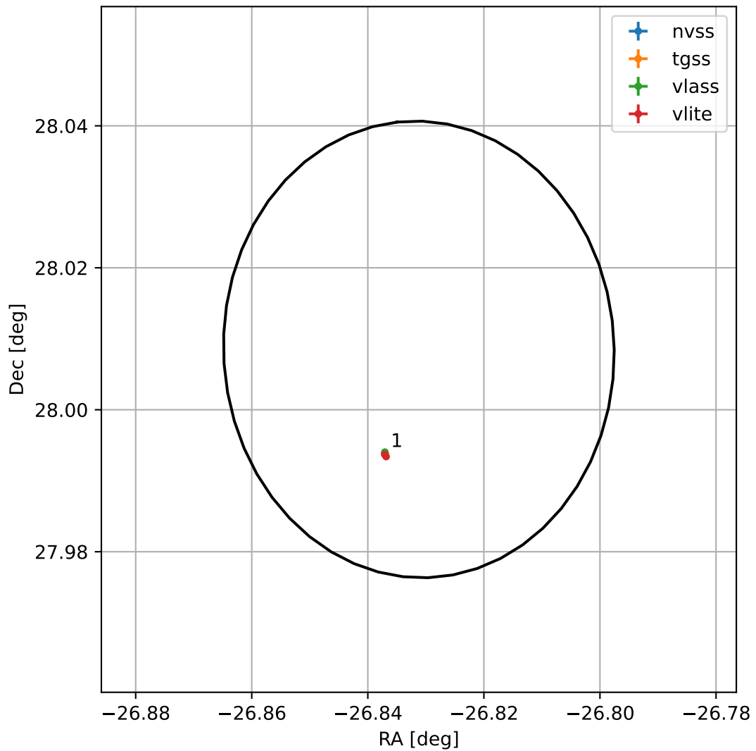
4FGL J2212.6+2800
