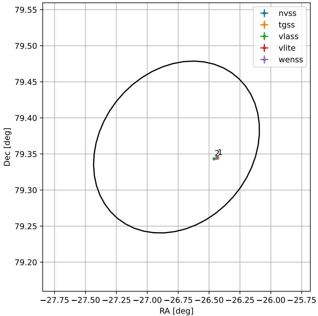
4FGL J2212.9+7921
