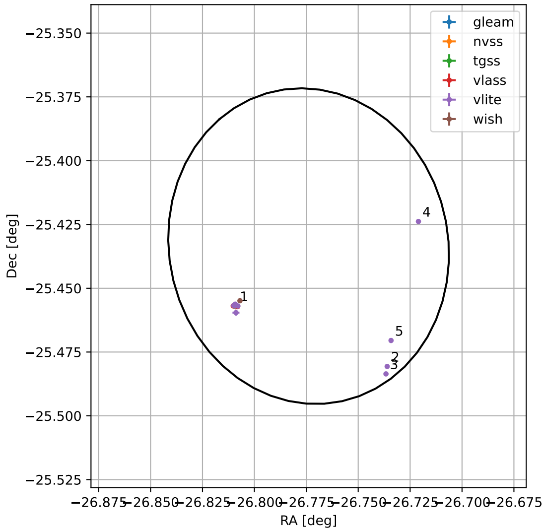
4FGL J2212.9-2526
