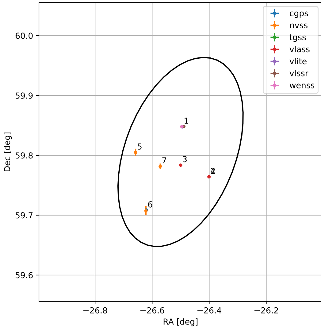
4FGL J2213.9+5948
