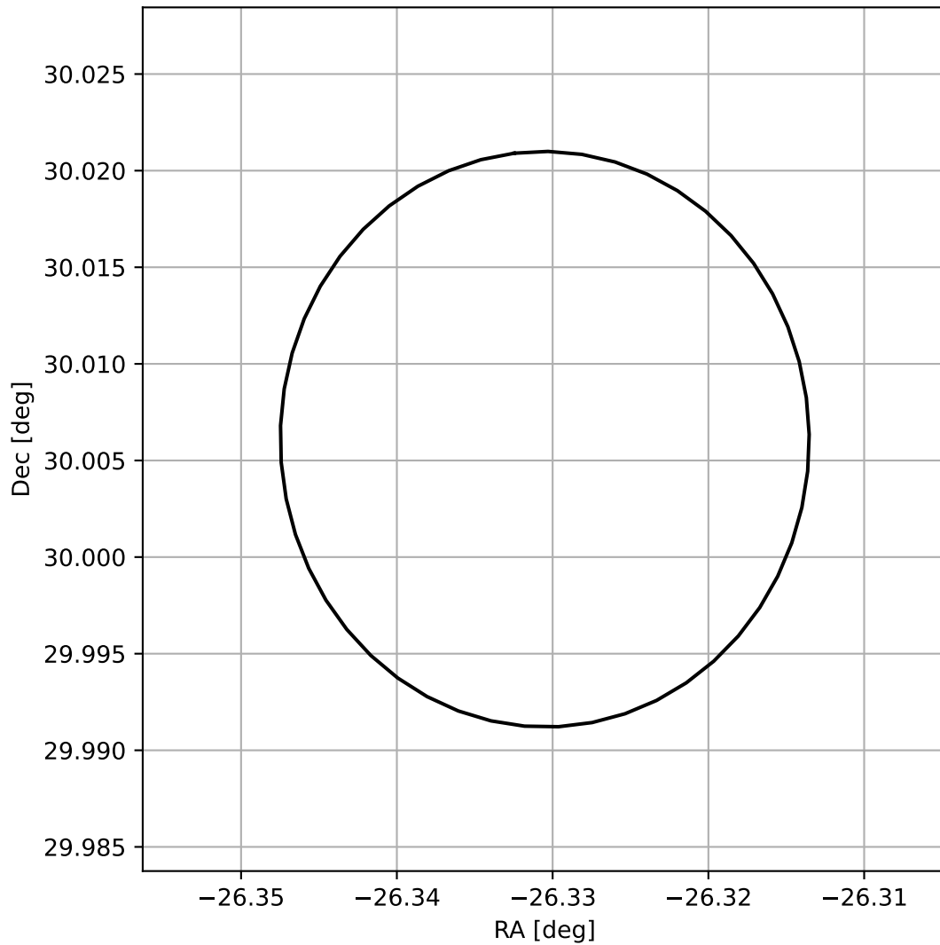
4FGL J2214.6+3000
