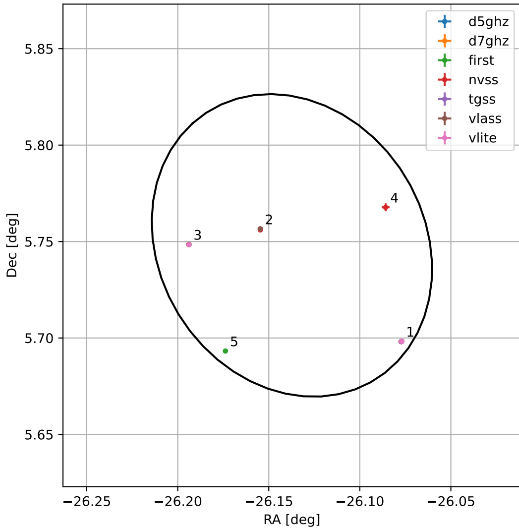
4FGL J2215.4+0544
