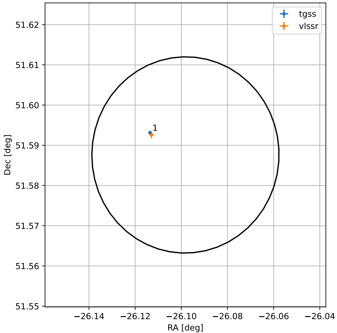
4FGL J2215.6+5135
