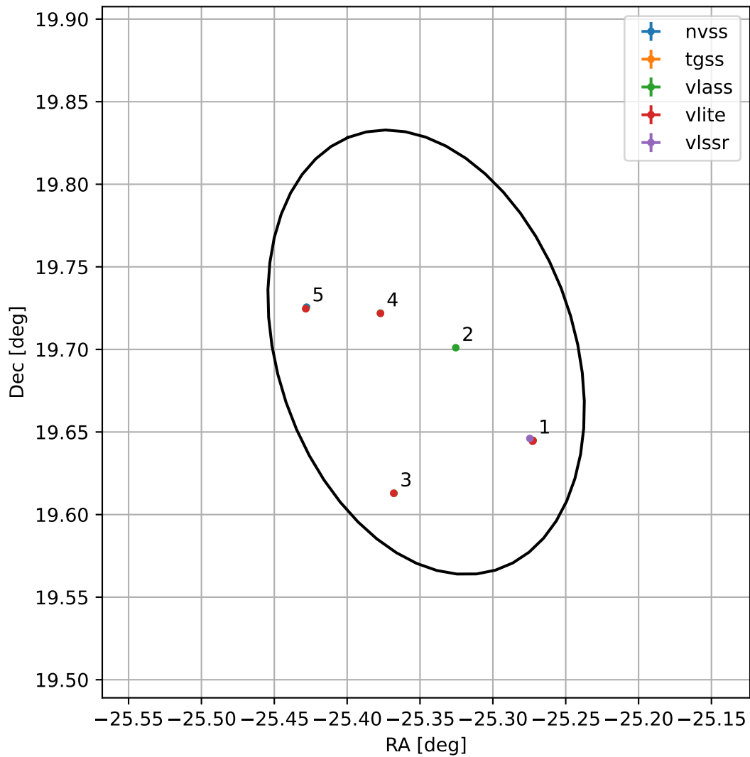
4FGL J2218.6+1941
