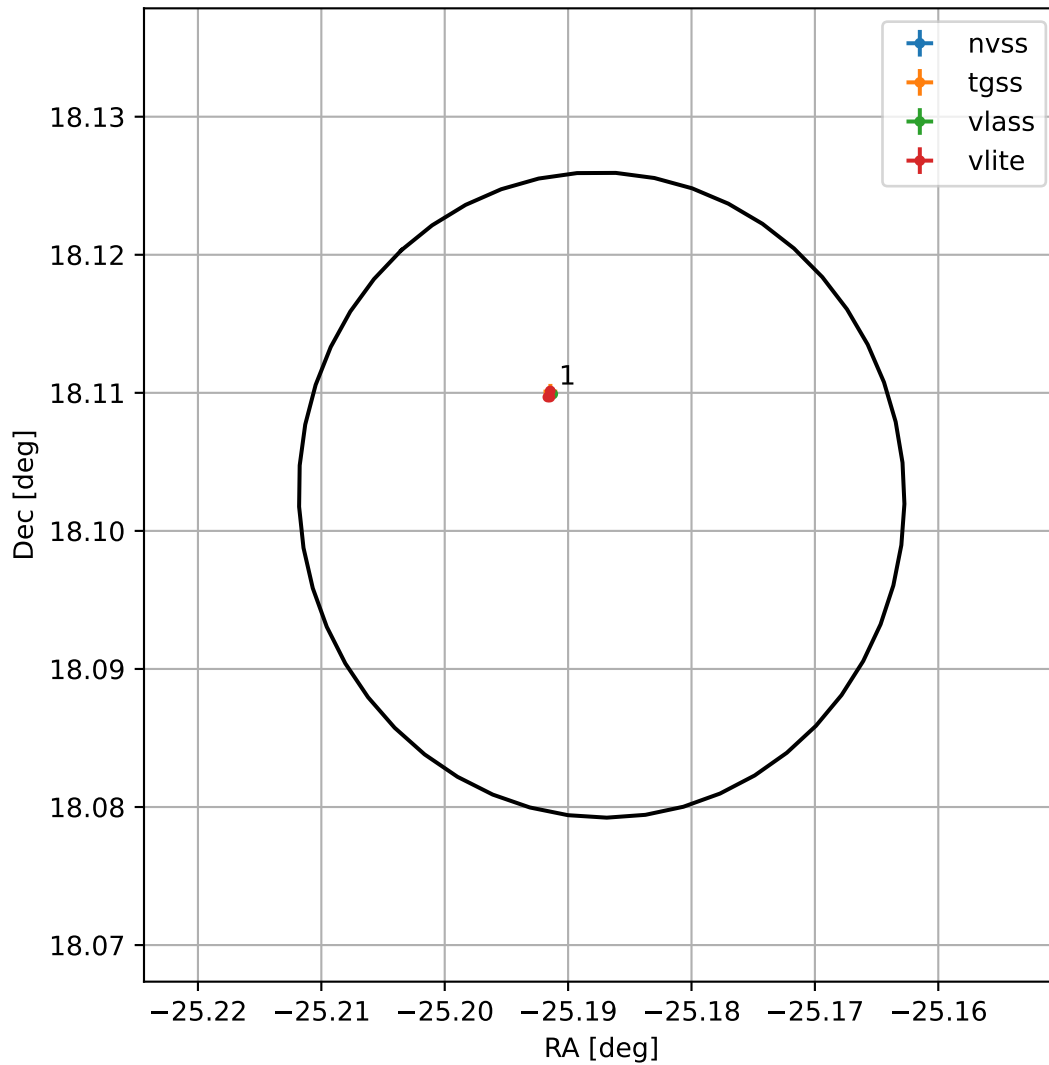
4FGL J2219.2+1806
