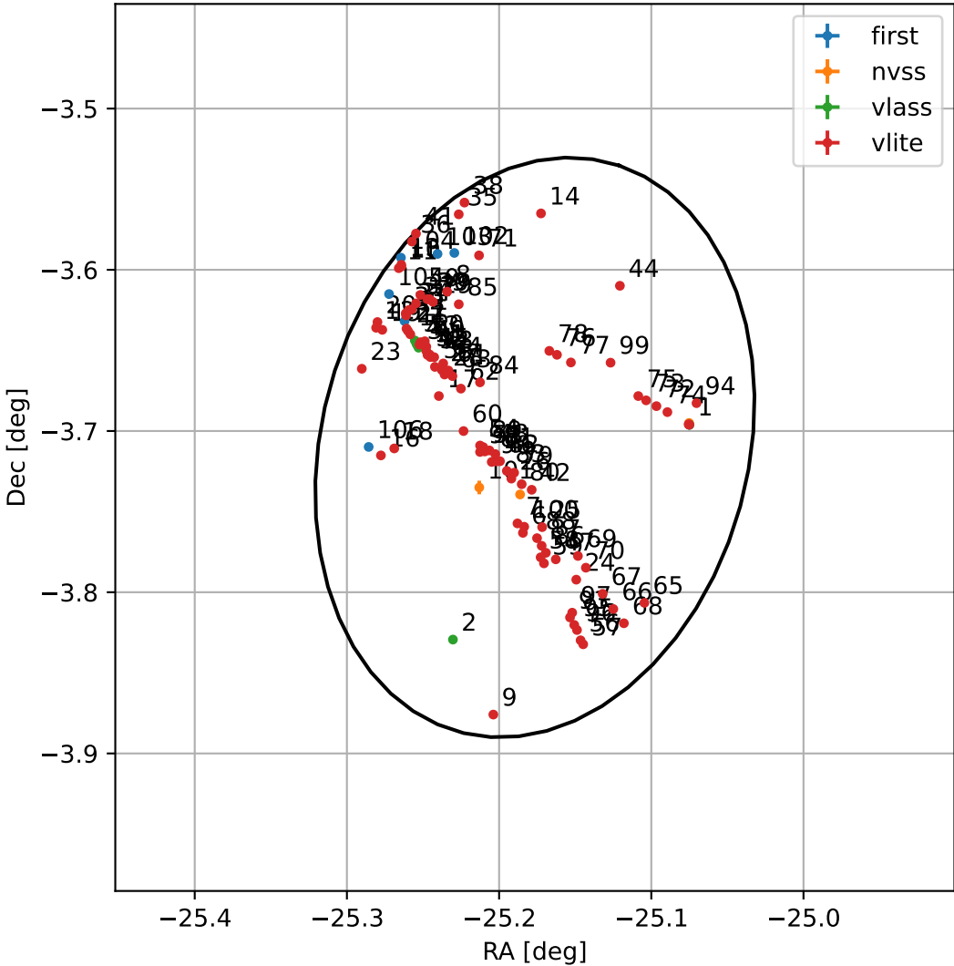
4FGL J2219.2-0342
