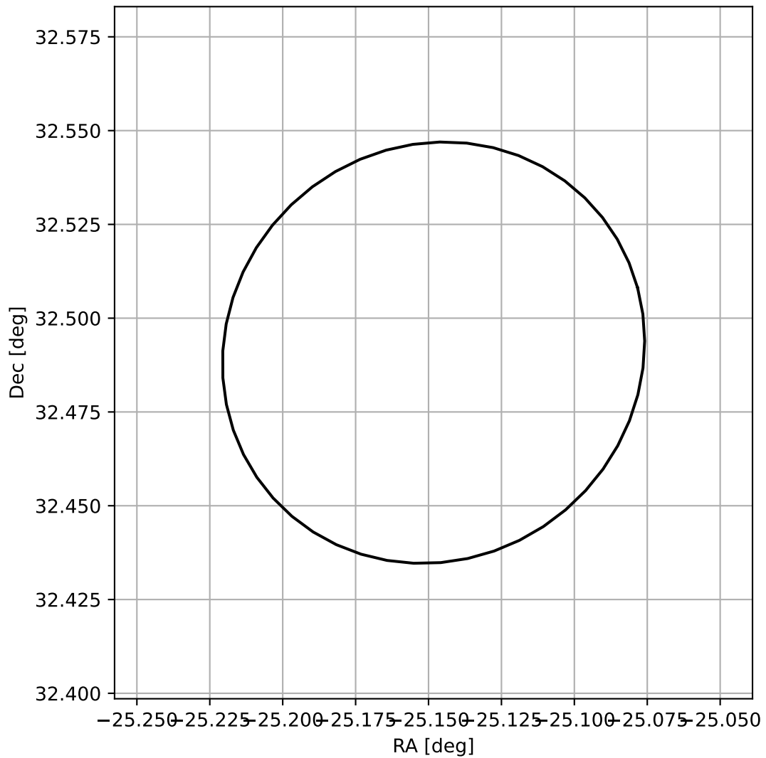
4FGL J2219.4+3229
