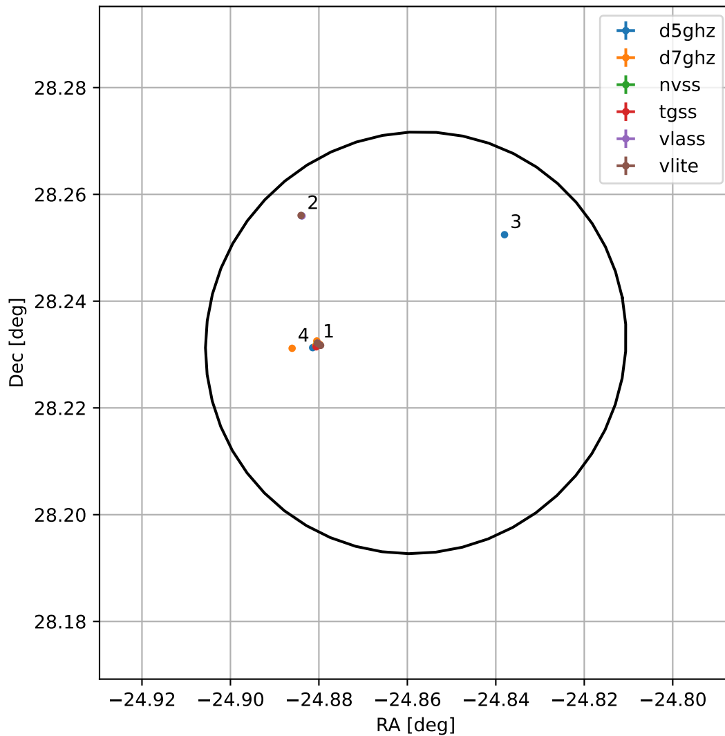
4FGL J2220.5+2813
