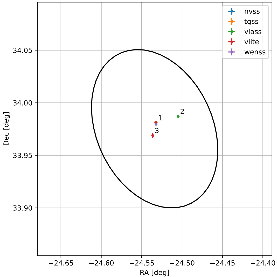
4FGL J2221.8+3358
