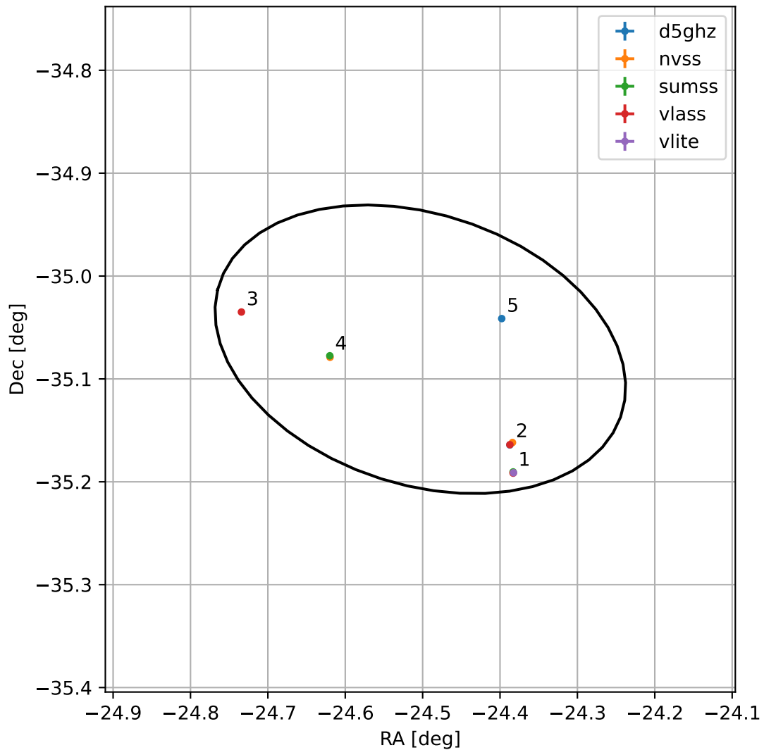
4FGL J2221.9-3504
